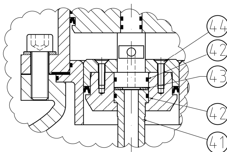
Scheme for DN100
